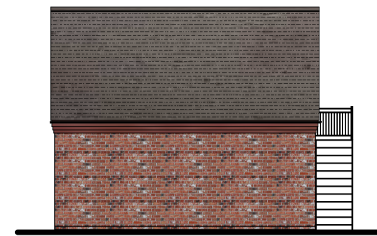
GARAGE SIDE (1:100)
